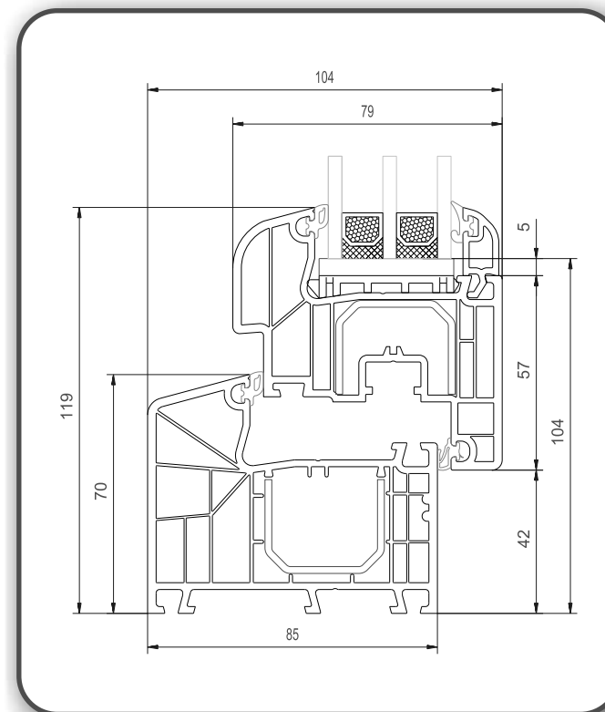
IDEAL MAX Round-line
